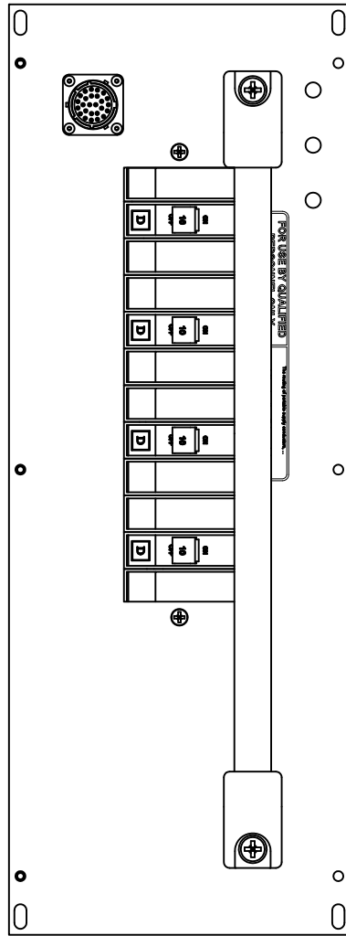
FRONT VIEW
