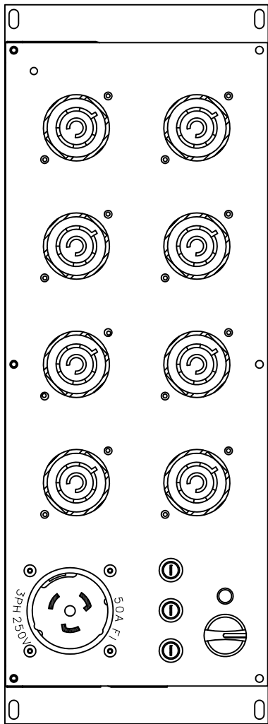
REAR VIEW
